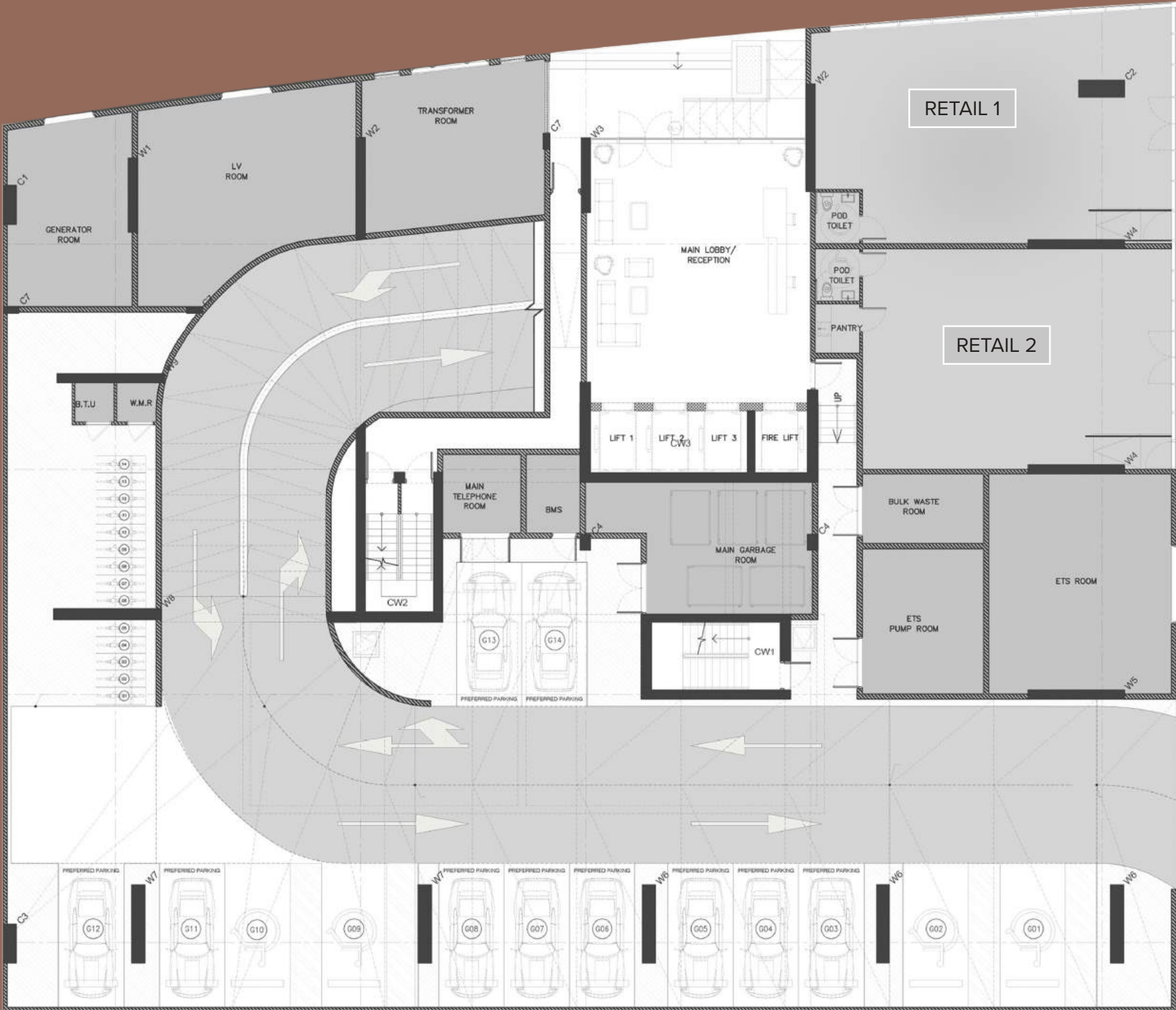
GROUND FLOOR
