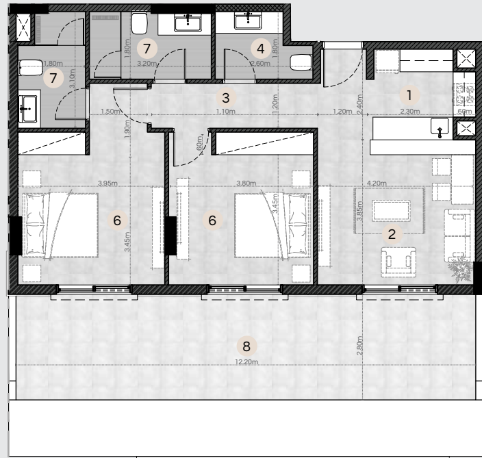
2 Bedroom Type 5-A 131.71m 2 (1,417.71ft 2 )
