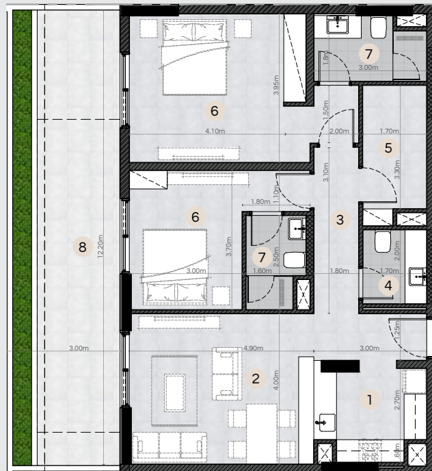
2 Bedroom Type 3-A 125.90m 2 (1,355.18ft 2 )
