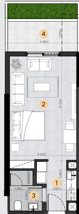
Studio Type 2-A 47.61m 2 (512.47ft 2 )
