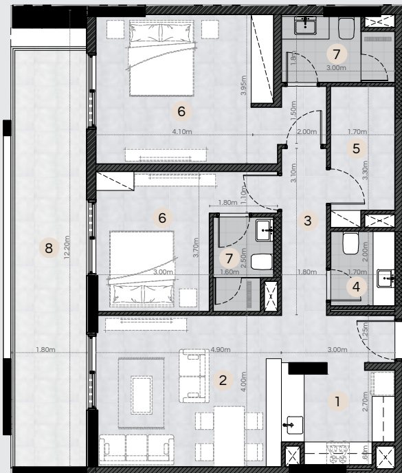
2 Bedroom Type 3-B 121.14m 2 (1,303.94ft 2 )
